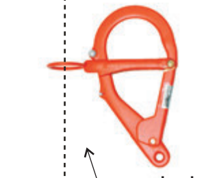
hook Ref.: DT 650 01 Weight: 0,75 kg Opening 75 mm
