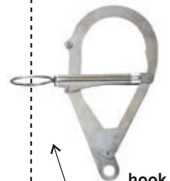
hook Ref.: DT 650 02 Weight: 0,60 kg Opening 75 mm
